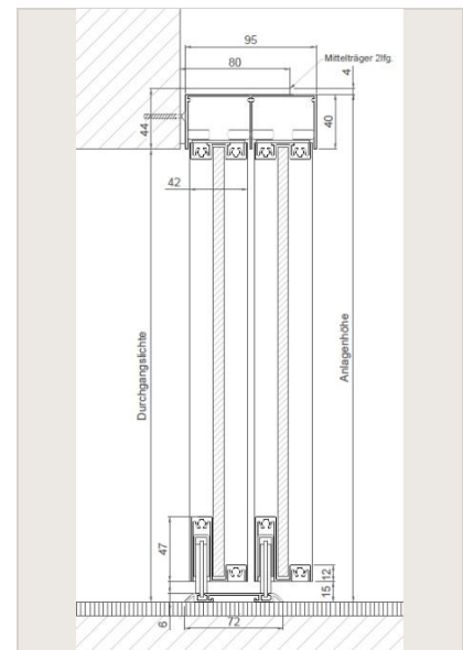
Deckenschiene Wandmontage
